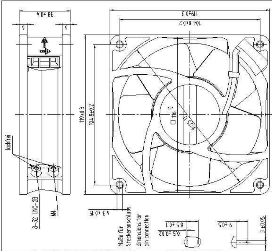
I) dimensions for assembly wall
